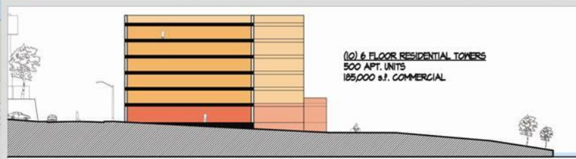
02 E. 112ND STREET- 6 FLR. TOWER SCALE: 1/8"=1'-0"
