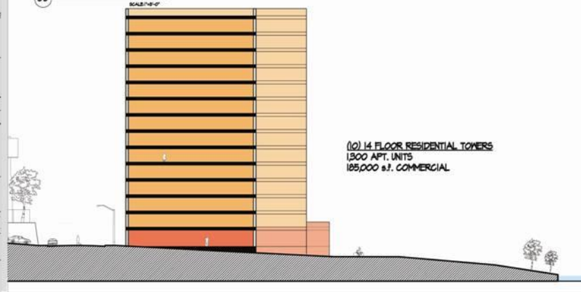
04 E. 112ND STREET- 14 FLR. TOWER SCALE: 1/8"=1'-0"
